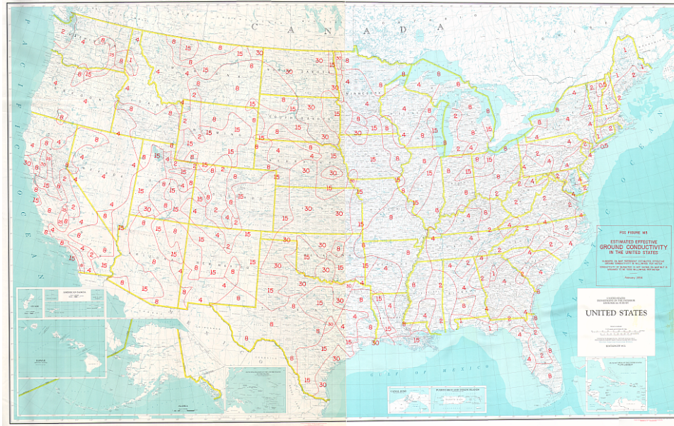
Figure B1: Ground conductivity
